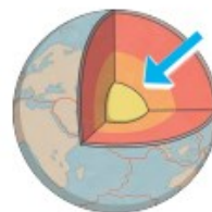
outer core
