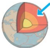
mantle
