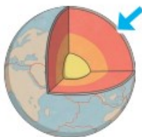
crust
