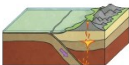
tectonic plate
