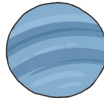
Neptune
